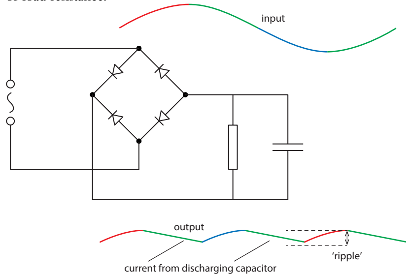
Figure 11.47 A capacitor in parallel to the load resistor smooths out the output voltage.
