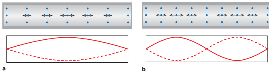
Figure 4.66 The first and second harmonics for a pipe with both ends closed.
