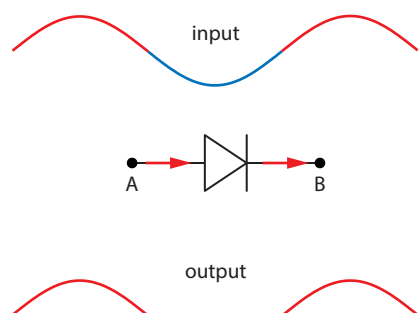
Figure 11.27 Half-wave rectification.
