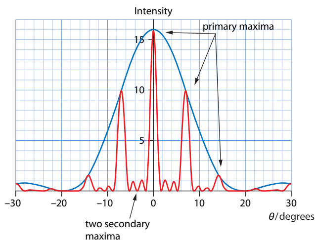
Figure 9.22 Intensity pattern for four slits.
